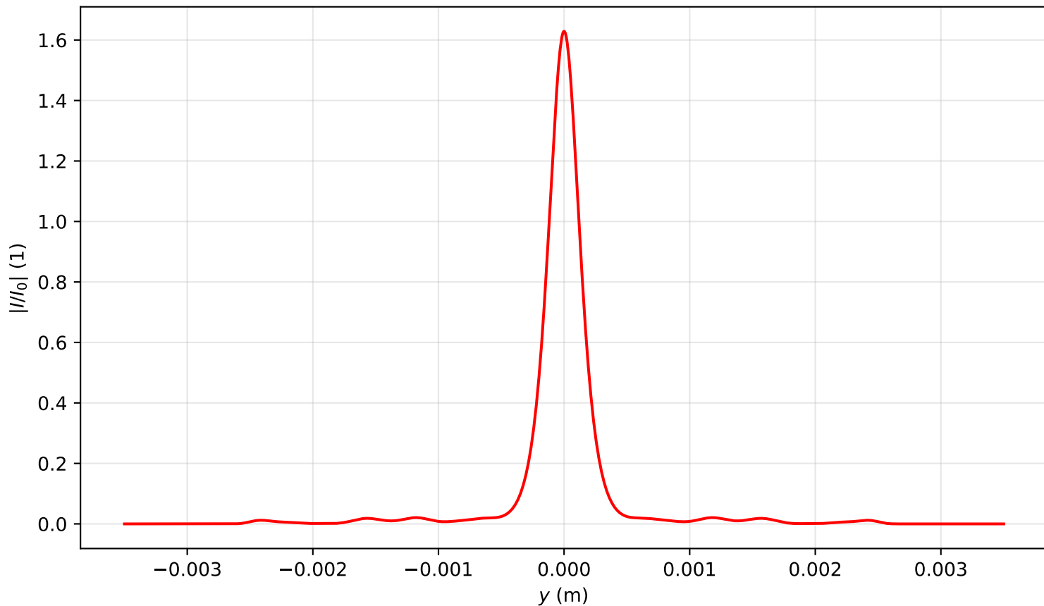
Intensity profile I(x=0, y, z=3.821)/I_0 , P_{in}=4.0P_{cr} , artificial time
